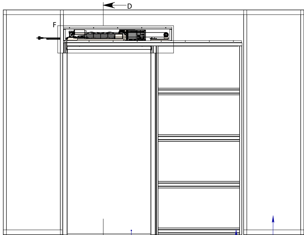
Front View
