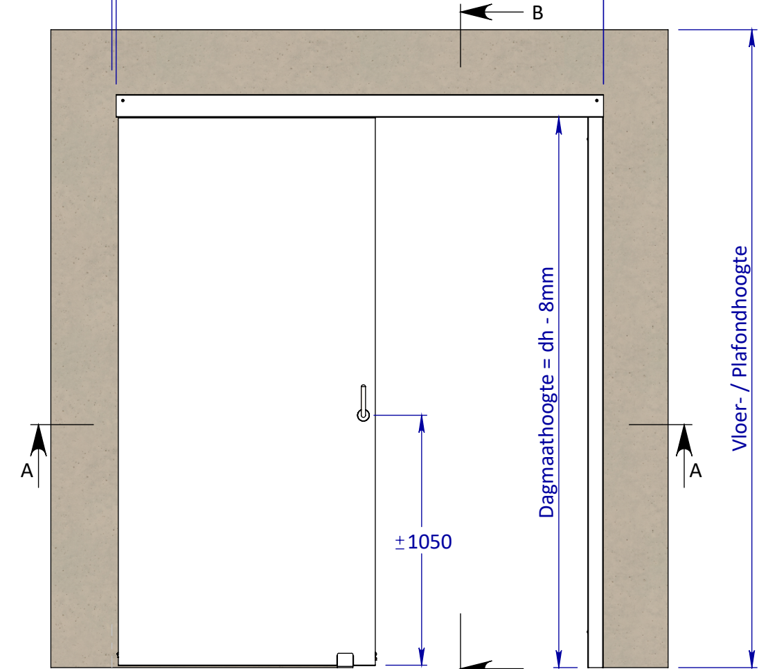
Front View
