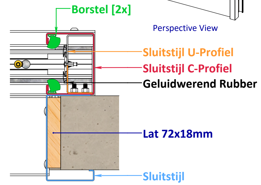
DETAIL C
