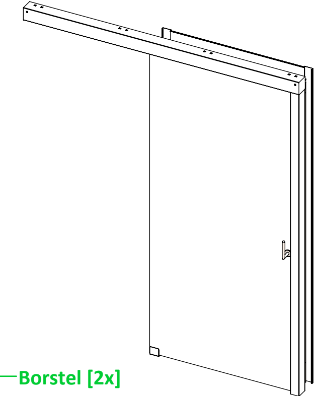
Perspective View
