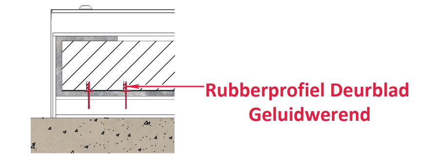
DETAIL D
