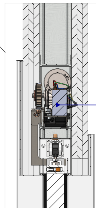
DETAIL E
