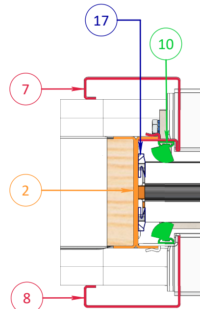
DETAIL C
