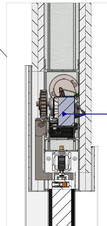
DETAIL E
