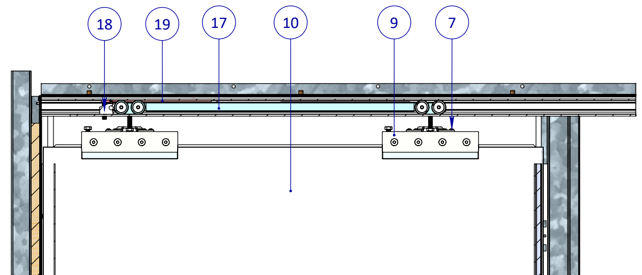
DETAIL D
