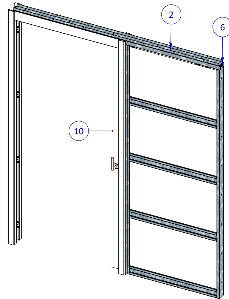
Exploded View
