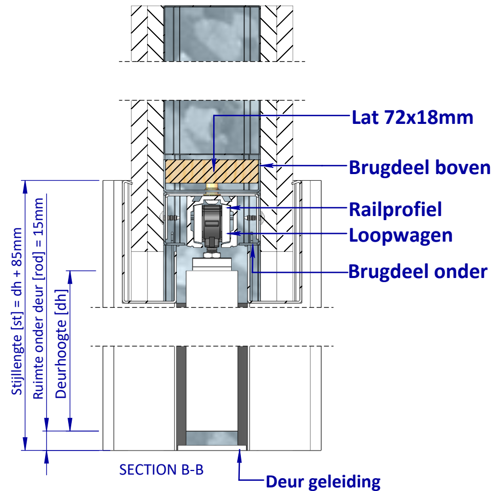
Right View
