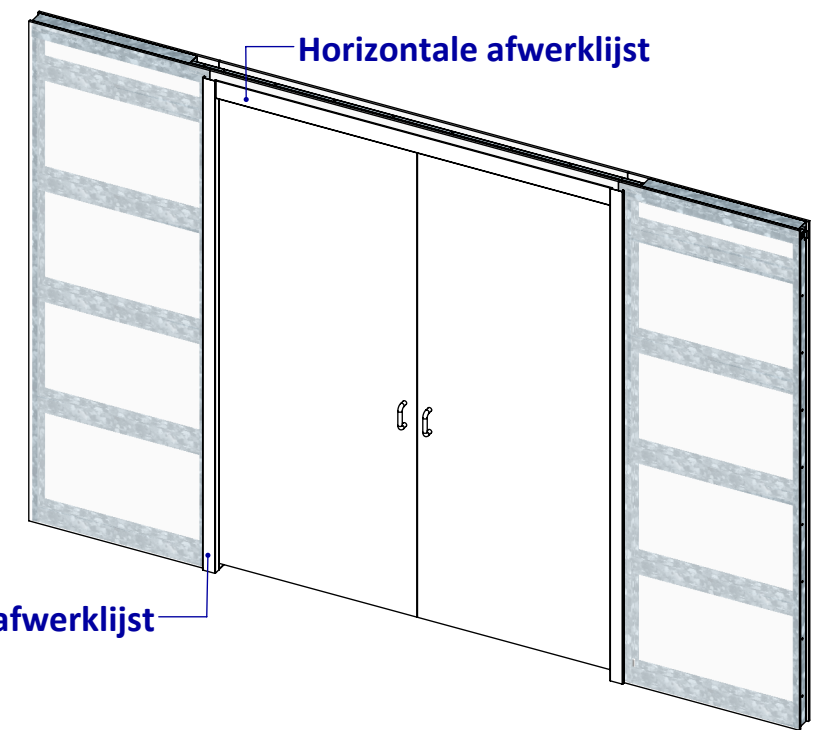
Perspective View
