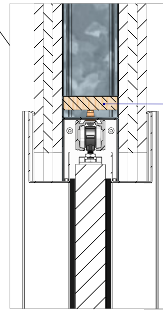
DETAIL E
