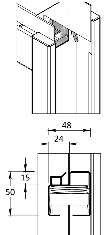
DETAIL F
