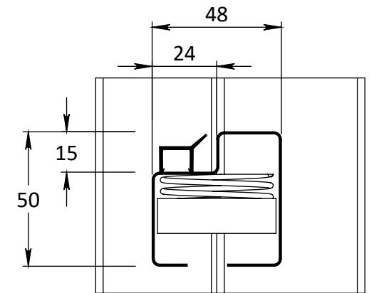
DETAIL D
