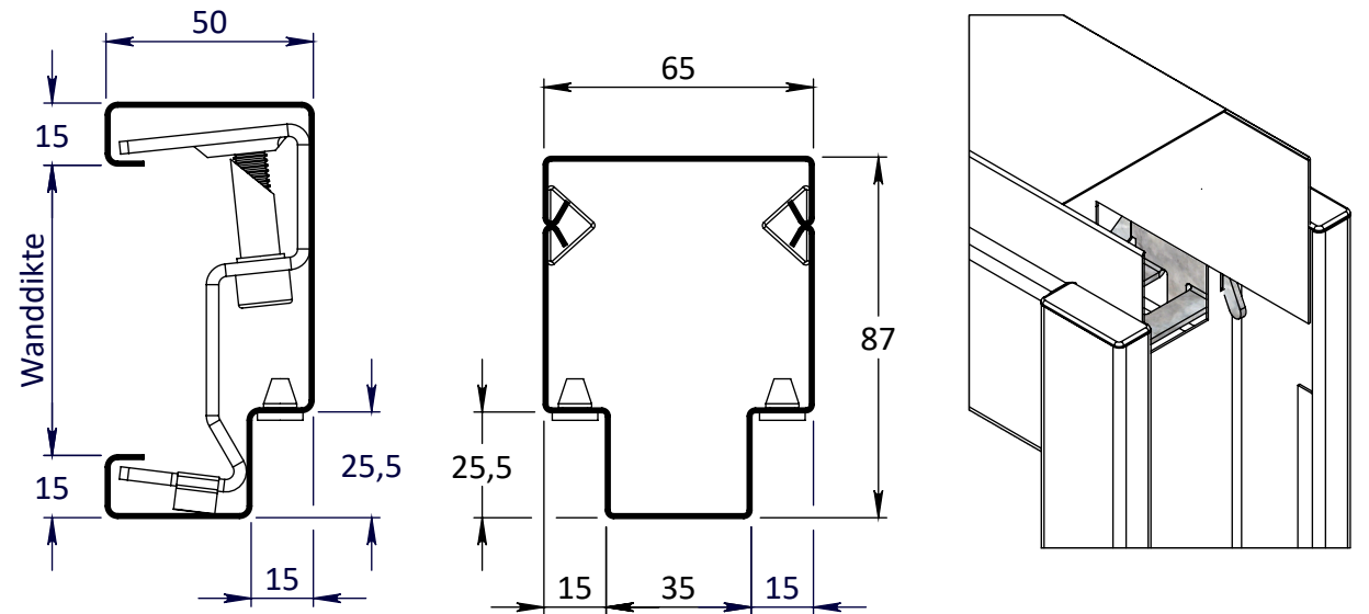
DETAIL C
