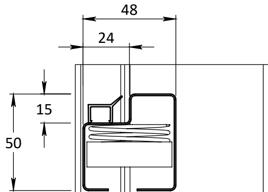
DETAIL D
