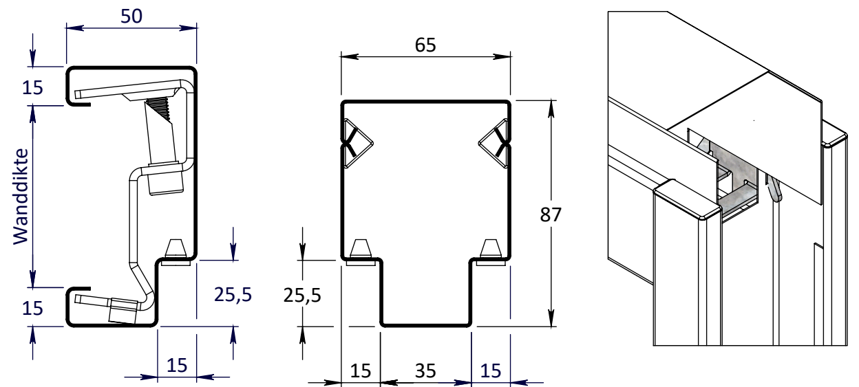
DETAIL C
