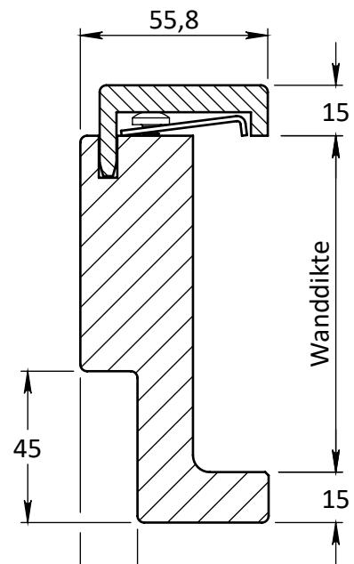
DETAIL C
